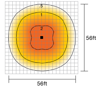
DISTRIBUTION PATTERN Bird's Eye View, Ceiling Mounted
